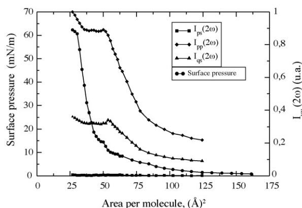
Fig. 3. Π–A isotherms and v polarized input and η polarized output light second harmonic intensity spectra ( I vη ) versus area.
