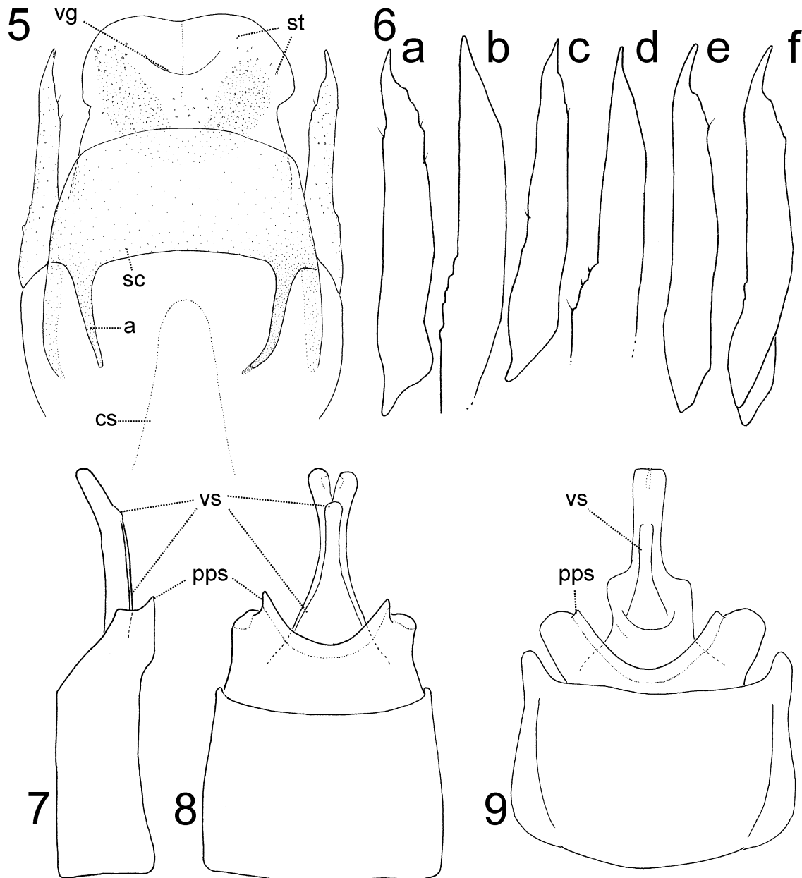
FIGURES 5–9. Caenis teipunensis sp. nov.: 5, male genitalia, v.v. (a=apophysis, cs=central sclerite, sc=styli-ger sclerite, st=small tubercles, vg=ventral groove); 6a–f, variations in forceps. Macunahyphes pemonensis sp. nov.; 7, male genitalia, l.v.; 8, same, v.v. Macunahyphes incognitus : 9, male genitalia, v.v. (pps= posterior projection of styli-ger, vs=ventral structure of penes).
