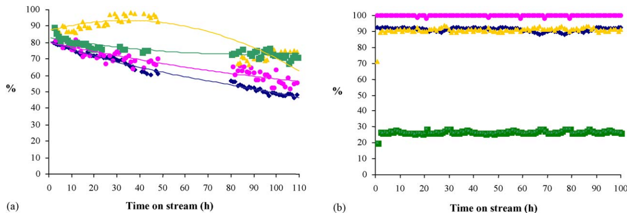
Fig. 5. Catalytic properties vs. time on stream. (a) C3 solid and (b) perovskite-like oxide, (◆) CH 4 conversion (%), (●) CO 2 conversion (%), (■) selectivity to H 2 (%) and (▲) selectivity to CO (%). W = 200 mg, GHSV = 24 L/(h g), CH 4 /CO 2 feed ratio \cong 1 , atmospheric pressure, T = 700 °C, gas mixture composition: CH 4 /CO 2 /N 2 = 1:1:8.
