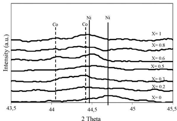
Fig. 8. XRD patterns of peaks respect to Ni 0 and Co 0 phases of LaNi 1-x Co x O 3 .
