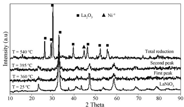
Fig. 6. LaNiO 3 crystalline phases as a function of the reduction temperature.
