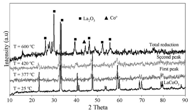
Fig. 7. LaCoO 3 crystalline phases as a function of the reduction temperature.
