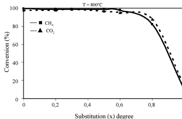
Fig. 10. CH 4 and CO 2 conversions on unreduced LaNi 1-x Co x O 3 at 800 °C.
