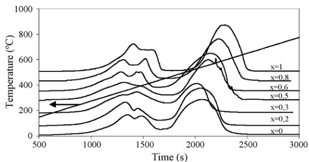
Fig. 5. LaNi 1-x Co x O 3 TPR profile.
